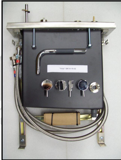
Photo 1. VOLA 14 Thermostatic mixer for bath filling and mixer with hand shower
